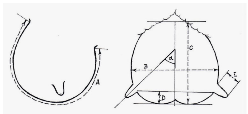
Figure 1: Morphological parameters measured on the udder and teats in French Lacaune dairy sheep. A: udder length (UL); B: udder width (UW); C: rear udder depth (RUD); D: cistern depth (CD); E: teat length (TL); \alpha : teat angle from the vertical (TA).
